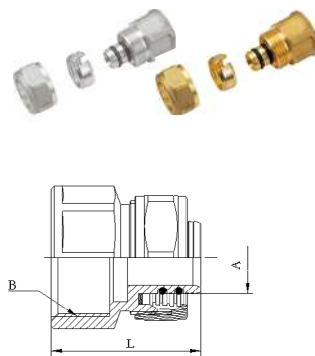
Female straight coupling
