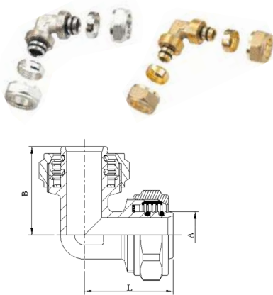
Elbow
