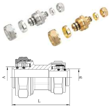
Reducing coupling
