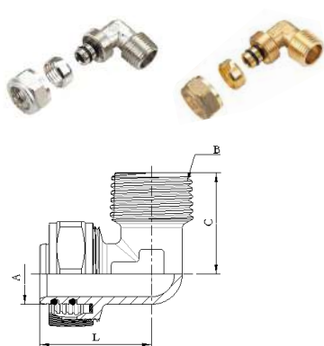
Male elbow
